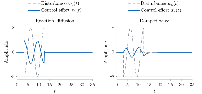
Figure 8: Disturbance and control effort for the reaction–diffusion equation (left) and damped wave equation (right).
