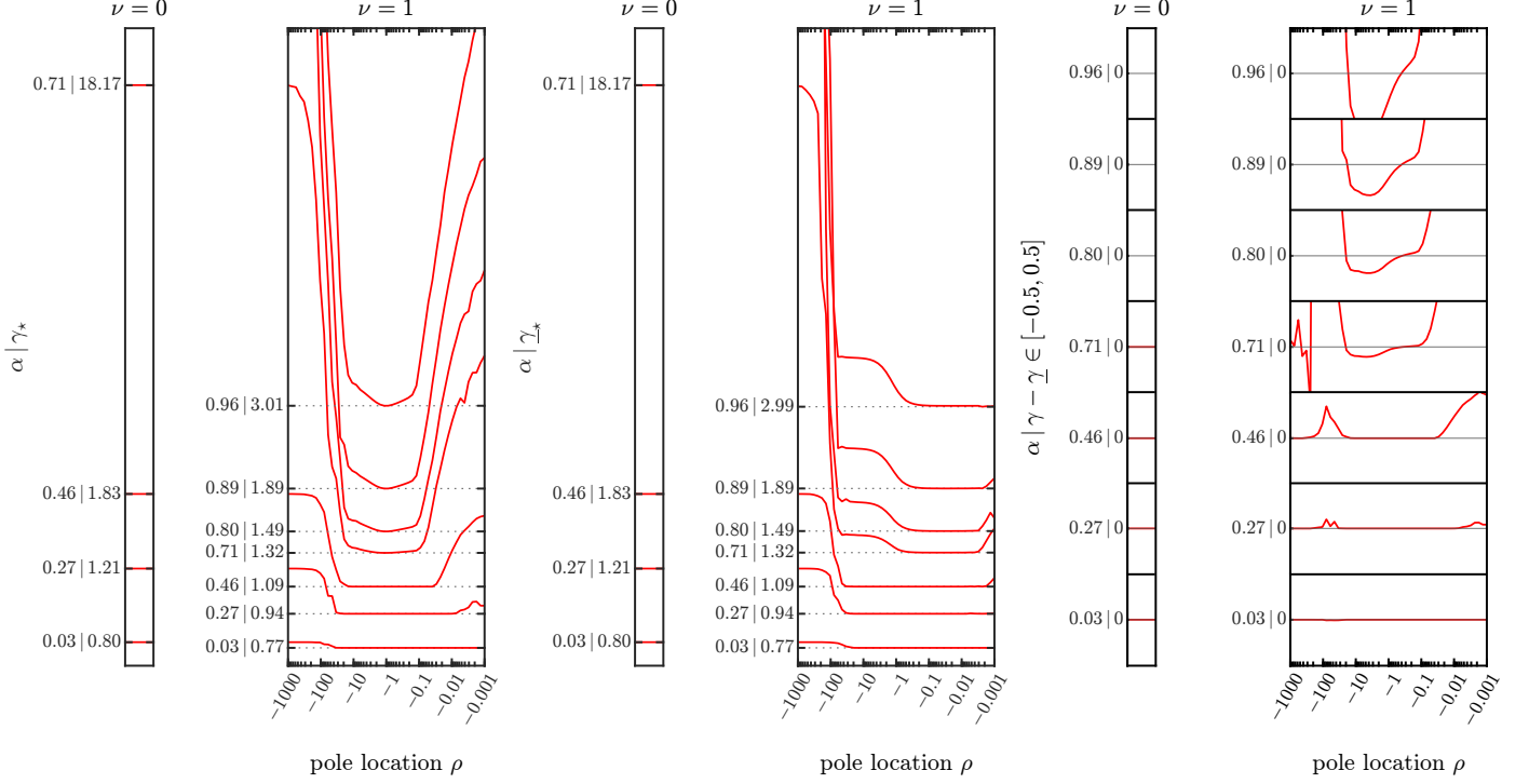
Figure 6: Reproduction of the sweep in [48, Fig. 7] for the coupled heat equations: primal analysis (left), dual analysis (center), and the difference \gamma - \bar{\gamma} between the primal and dual bounds (right). The figure highlights two main observations. First, even when using a lifted finite-dimensional filter for the dynamic IQC, the choice \nu = 1 yields substantially smaller values of \gamma than the static case \nu = 0 . Second, the dual analysis produces lower values of \gamma than the primal analysis. This indicates that, for the chosen IQC parameterization, the dual formulation yields less conservative bounds and allows the small-gain bound on G_0 to be pushed closer to \rho = 1 . This difference is possible because the problem is formulated such that \Theta need not coincide with \mathbf{D}(\Theta) , so the primal and dual analyses need not yield identical bounds under the same lifted finite-dimensional filter parameterization, which may be better suited to the dual system than to the primal system.
